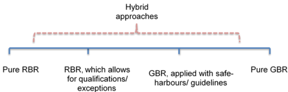
Figure 1: Spectrum of RBR and GBR
